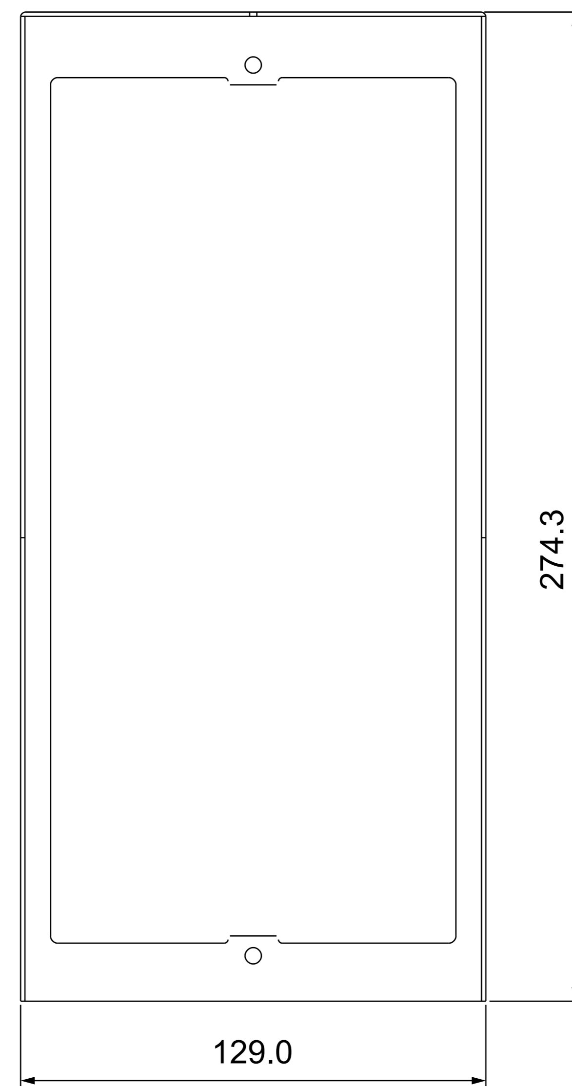
1 FRONT VIEW
