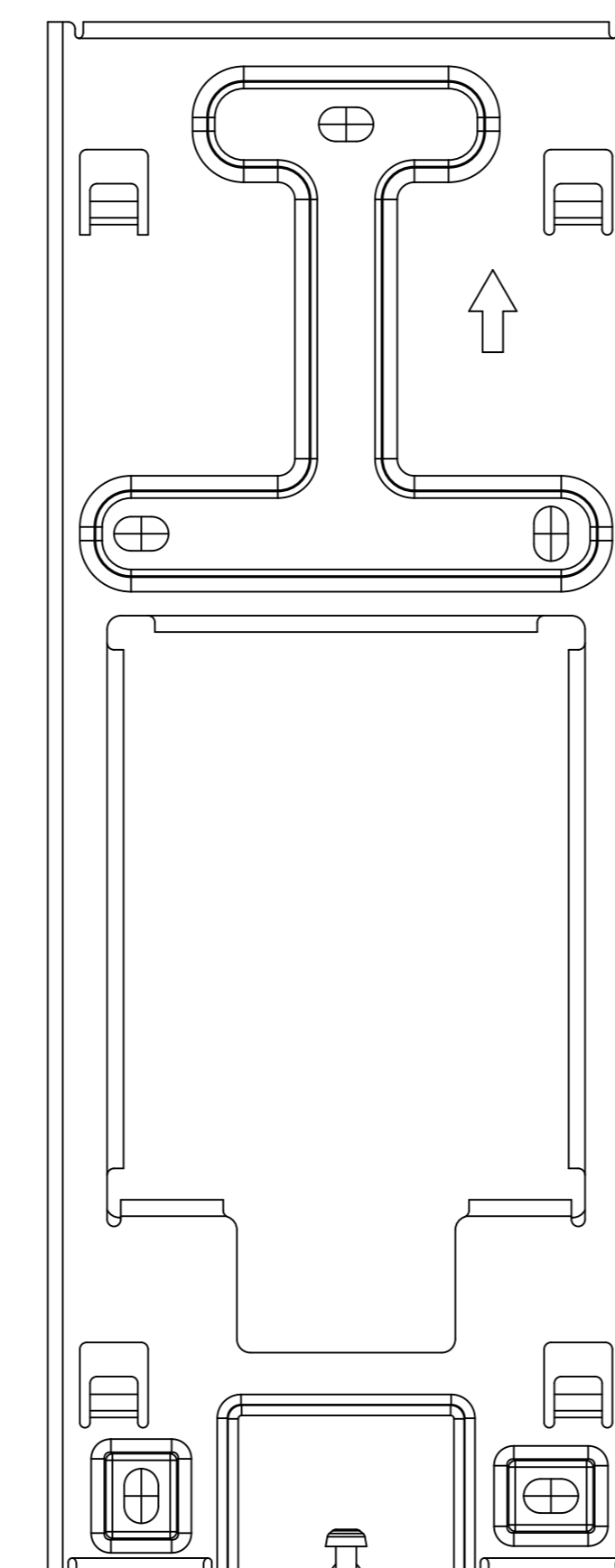
② FRONT VIEW:WALL MOUNTING BRACKET PLACEMENT
