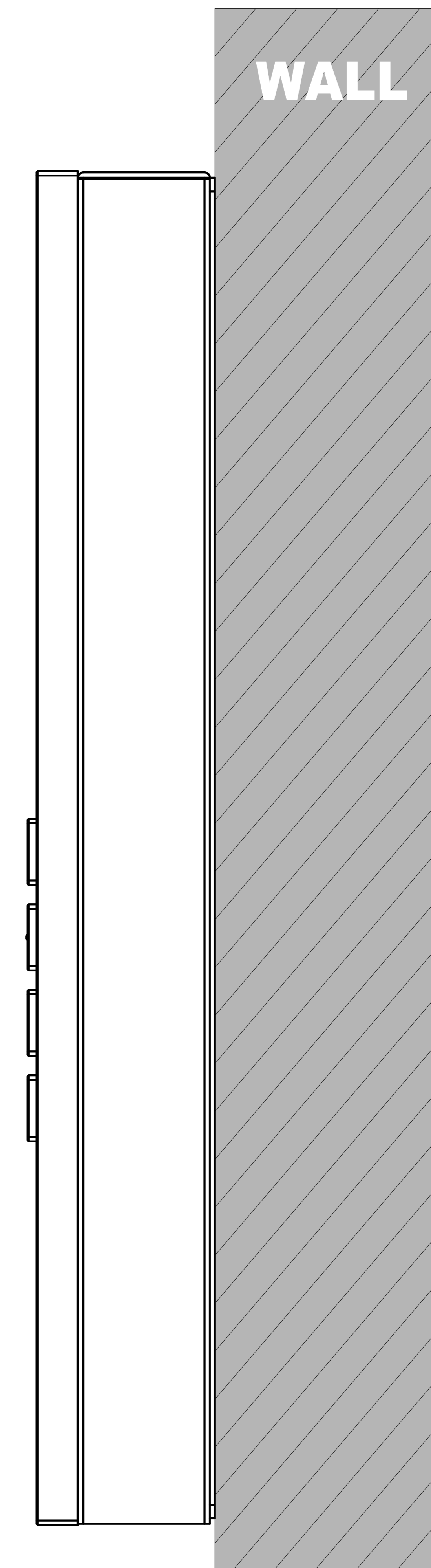
③ SIDE VIEW:INTERCOM ON WALL
